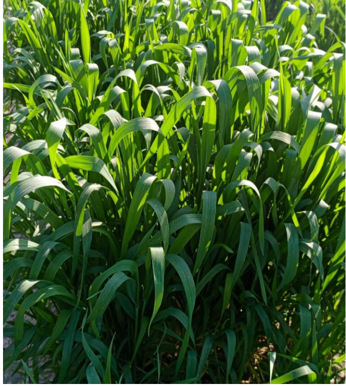
CRISPR-CAS9 Edited
